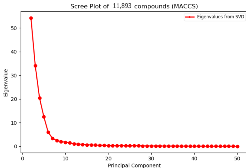
Fig S1. Scree plot for the transformed vector space using 11,893 compounds.
